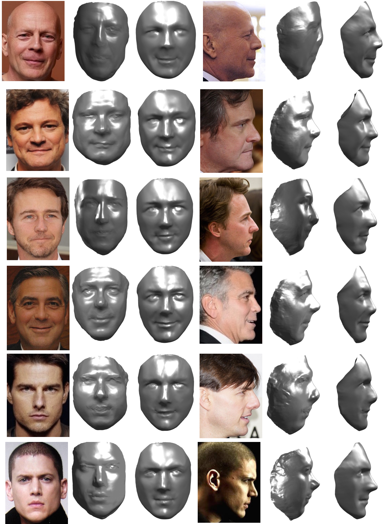
Figure 6: Comparison results of different individuals between the state of the art technique by Roth et al. [RTL15] and our approach. (The 2nd and 5th column are the results from the code made available from [RTL15], the 3rd and 6th column are our results.)
