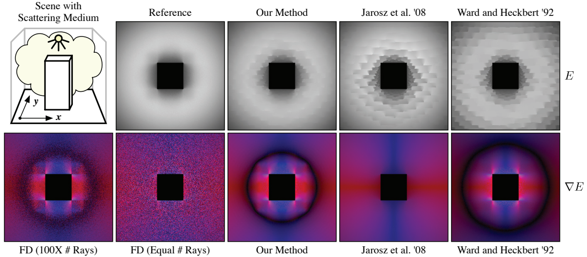
Figure 5: This modification of the scene from Figure 3 contains a spot light and a scattering medium. Our gradient formulation obtains accurate results by taking into account the medium and surface-medium occlusions, whereas previous methods ignore these effects.
