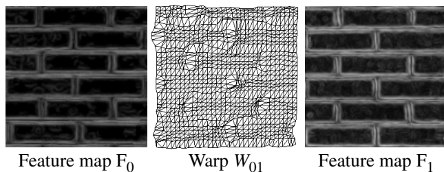
Figure 2: Visualization of the dense warp field W_{01} between two feature maps F_0 and F_1 .
