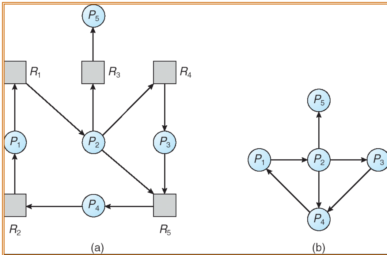
Resource-Allocation Graph
