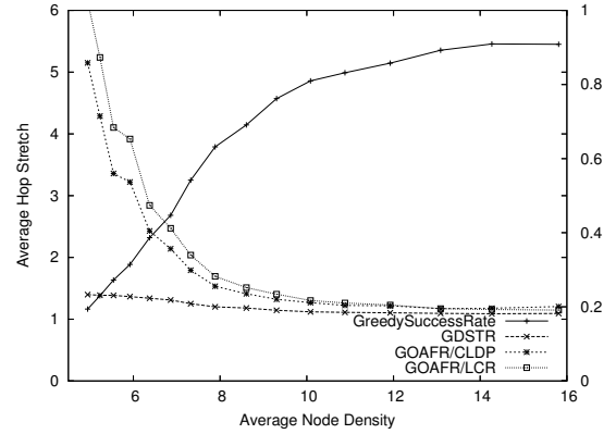
Figure 20. Stretch, N/2 obstacles, 400 nodes.
