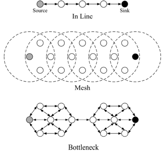
Figure 8: Three topologies used in Simulation Experiment
