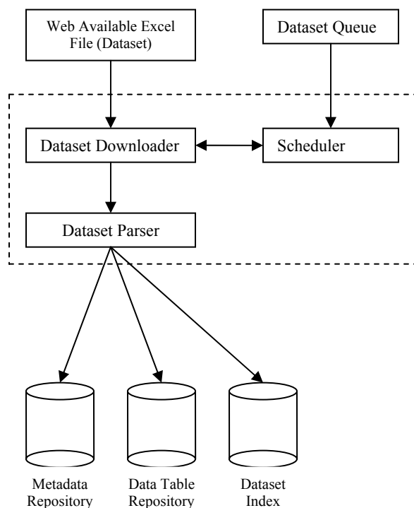
Figure 5: Dataset Downloader and Parser Architecture.
