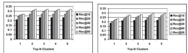
Figure 5: Recall@K for GOV2/P1000 (left) and GOV2/P5000 (right).
