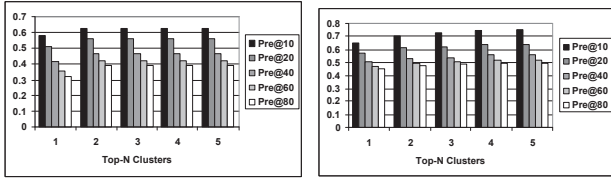
Figure 6: Precision@K for GOV2/P1000 (left) and GOV2/P5000 (right).
