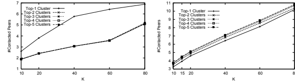
Figure 7: Number of contacted peers for GOV2/P1000 (left) and GOV2/P5000 (right).
