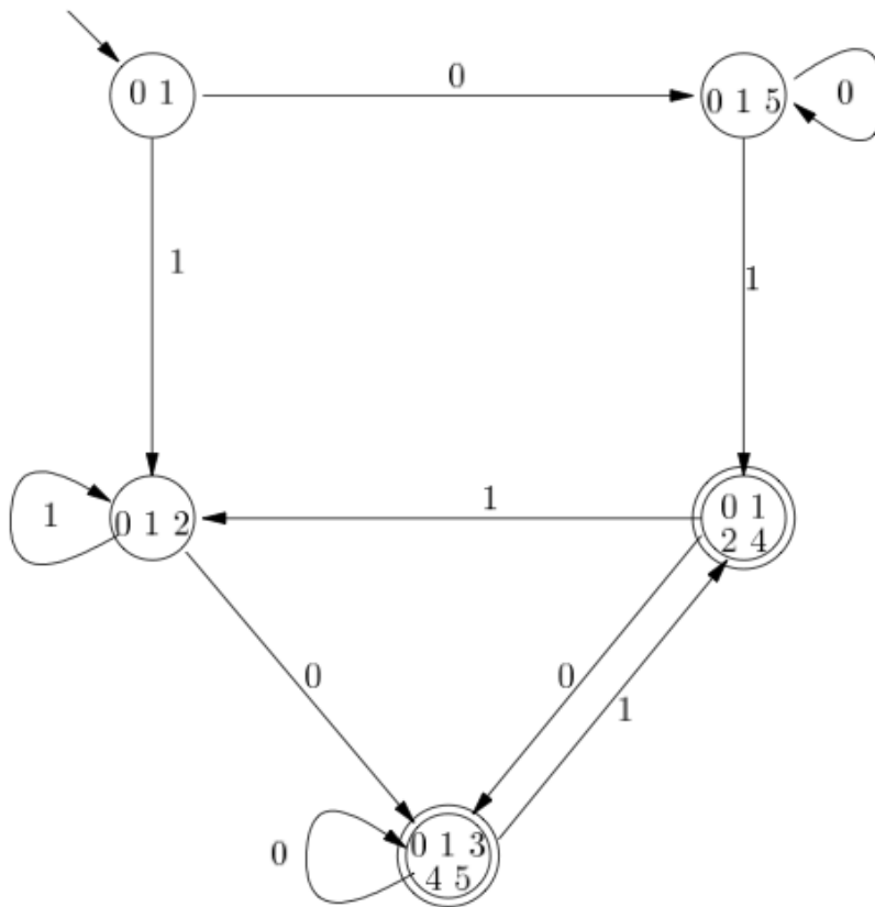
Figure 3: DFA
