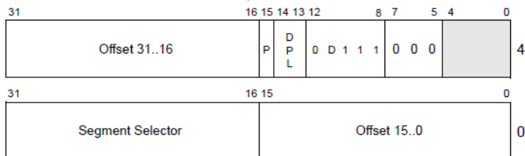
Trap Gate
