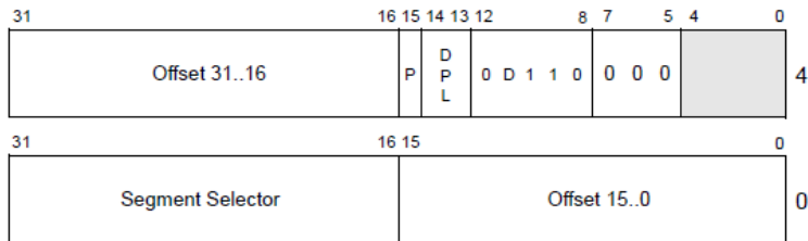
Interrupt Gate
