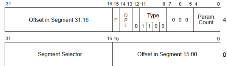
Call Gate
