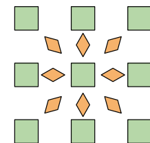
Fig. 2: LeanMD Decomposition
