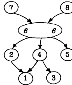
Topological numbering after cycle collapsing. Figure 3.
