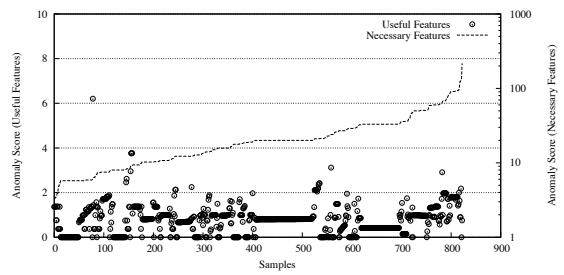
Figure 2: Breakdown of the anomaly score for samples in the known-bad datasets by feature category.
