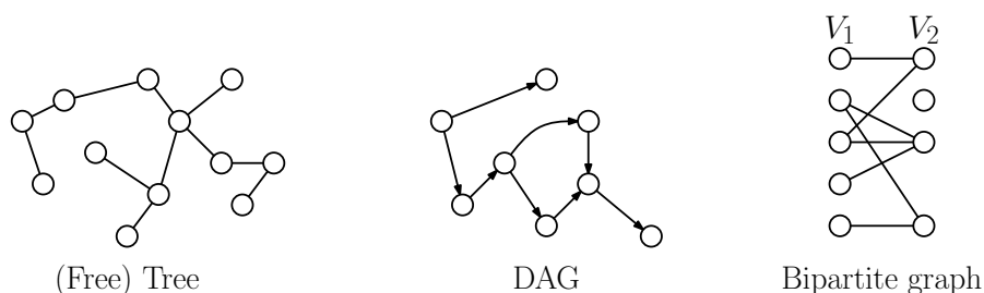
Fig. 2: Illustration of common graph terms.
