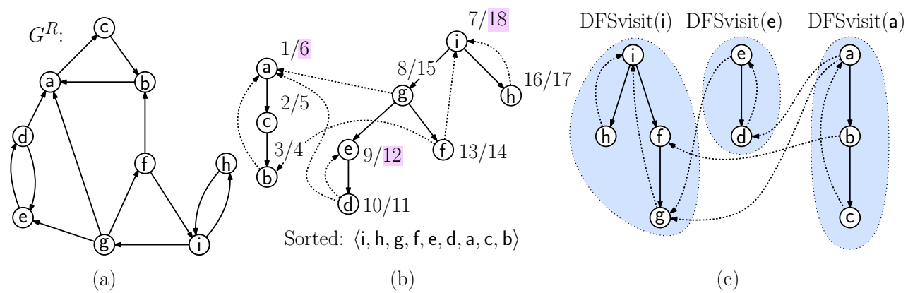
Fig. 5: Strong components and DFS.
