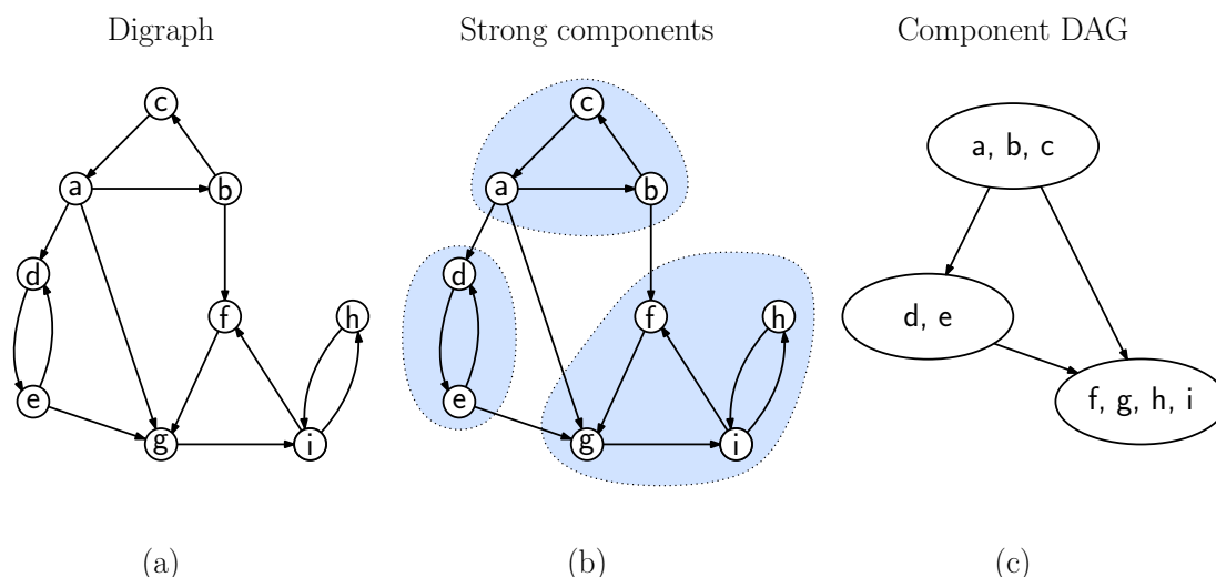
Fig. 4: Strong components and the component DAG.
