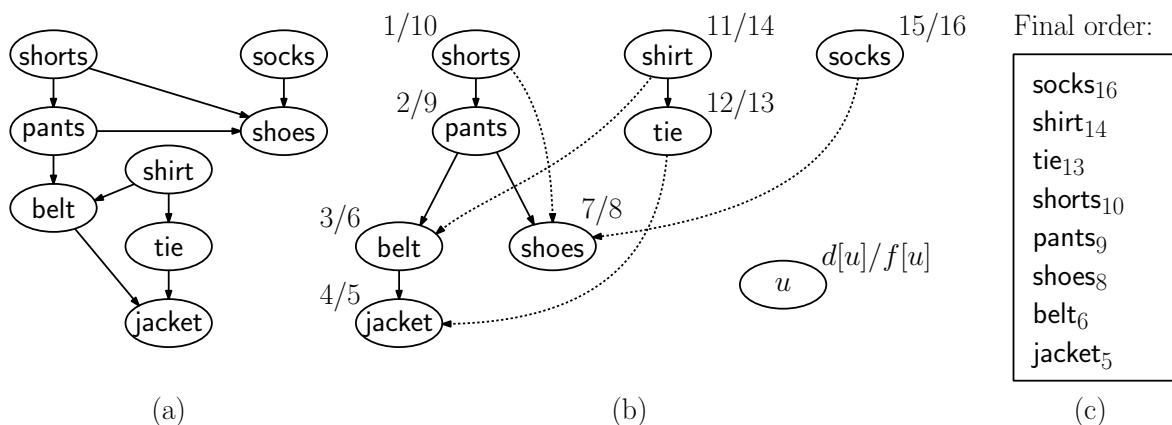
Fig. 2: Topological sorting example.
