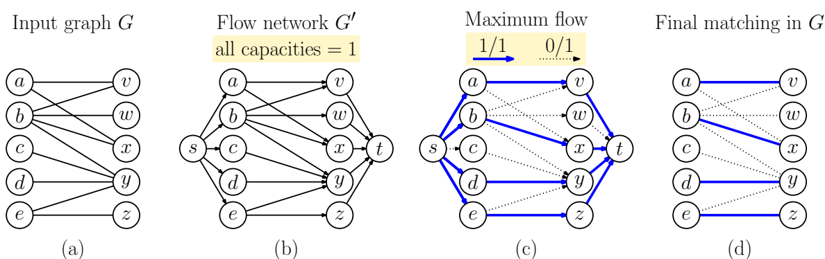
Fig. 5: Reducing bipartite matching to network flow.
