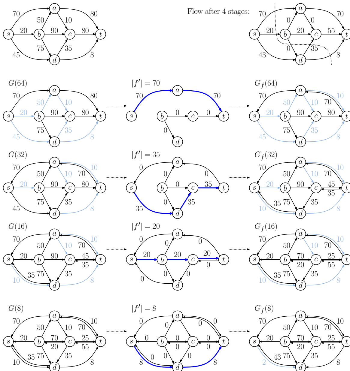
Fig. 3: The first four stages of the scaling algorithm for network flow. Note that at each stage, the value of the augmenting flow f' is at least \Delta . (The algorithm will run for G(4) , G(2) , and G(1) , but no changes to the flow will occur.)
