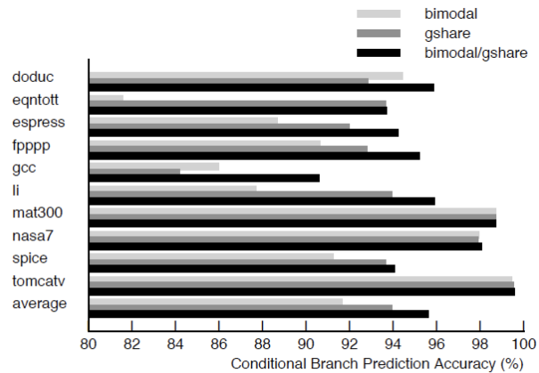
Figure 13: Combined Predictor Performance by Benchmark
