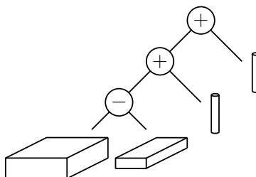
Fig. 2: CSG Tree.
