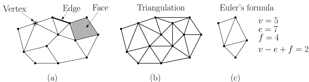
Fig. 5: Planar graphs and Euler's formula.
