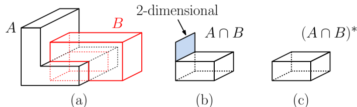
Fig. 3: (a) A and B , (b) A \cap B , (c) A \cap^* B .
