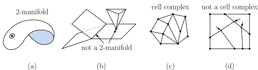
Fig. 4: 2-Manifolds and cell complexes.
