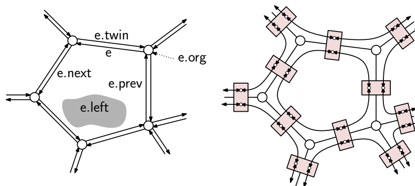
Fig. 6: Doubly-connected edge list.
