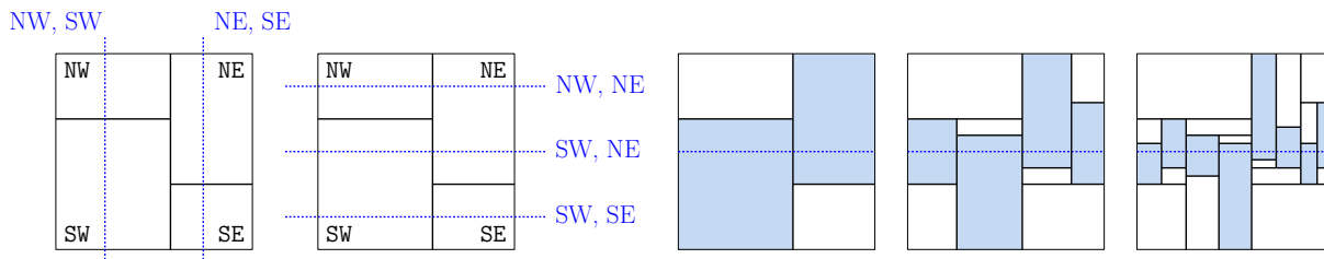
Fig. 6: An axis-parallel line in 2D can stab at most two out of four cells in two levels of the kd-tree decomposition. In general, it stabs 2^i cells at level 2i .
