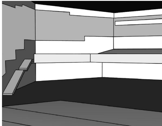
Acoustic Geometry
