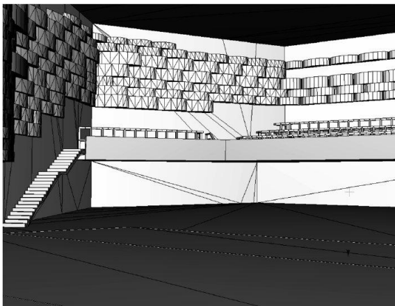
Visual Geometry
