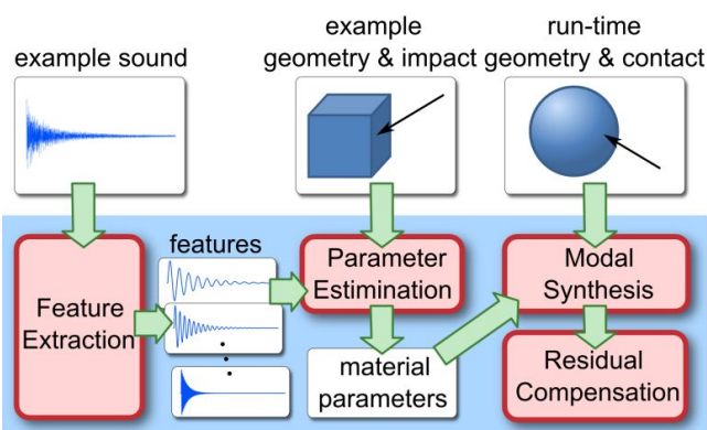
From “Example-Guided Physically Based Modal Sound Synthesis”
