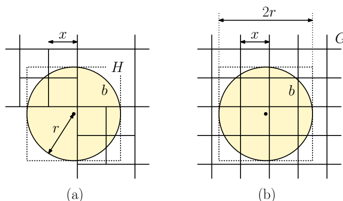
Fig. 8: Proof of the Packing Lemma.
