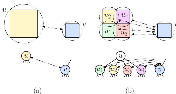
Fig. 6: WSPD recursive decomposition step.
