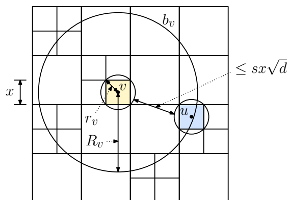
Fig. 7: WSPD analysis.
