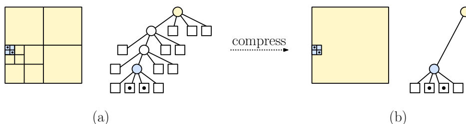
Fig. 5: Compressed quadtree: (a) The original quadtree, (b) after path compression.
