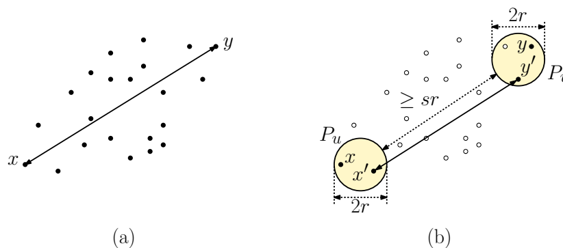
Fig. 3: Approximating the diameter.
