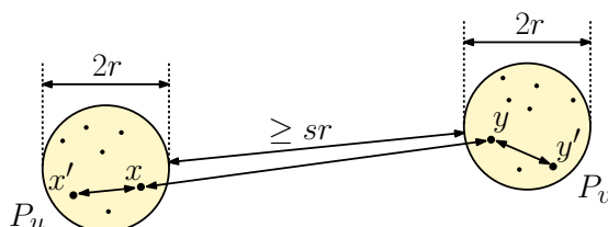
Fig. 2: WSPD Utility Lemma.
