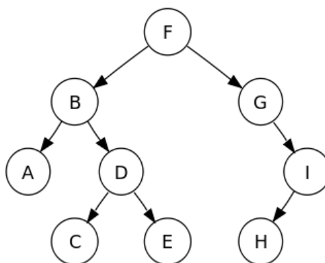
Figure 14.2: Binary Search Tree
