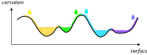
Figure 3: The watershed algorithm: First, we assign unique labels (patch IDs) to local minimums. Next, imagine that we place a drop of water at a vertex. The water drop will flow to the local minimum. We assign the label of the local minimum to the vertex where the water-drop was placed. We repeat this for each vertex.
