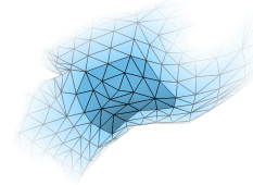
Figure 6: Visualization of weights for blending illumination from a patch. The dark area in the middle shows the patch, and the progressively whiter colors outside the patch show the weight values diminishing away from the patch boundary.
