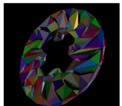
(l) \epsilon = 3\ 3/4\% , 716 triangles
