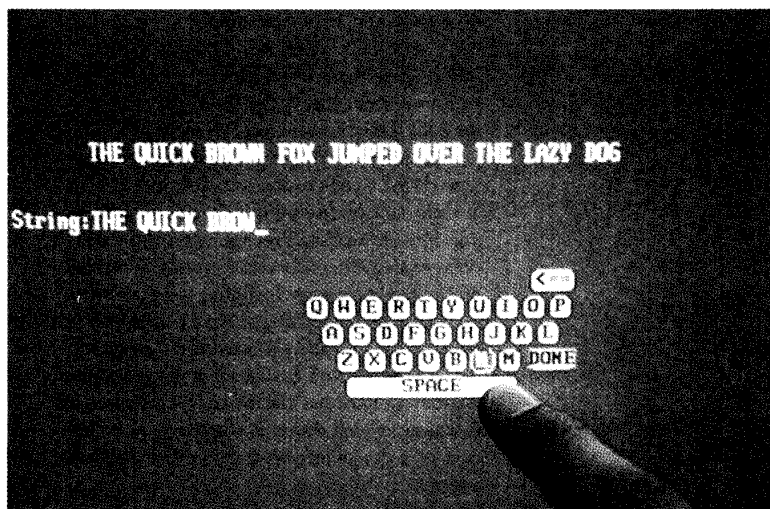
Figure 5. A touch-screen keyboard. Although slower than a traditional keyboard, it works well for note-taking, forms-entry, and other applications that require small amounts of input in a portable or small device.
