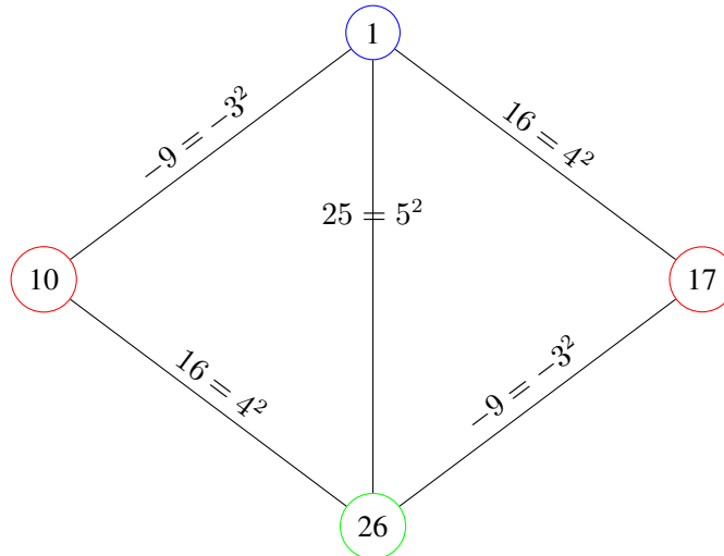
Figure 4. In any proper (x^2, 3) -coloring, \text{COL}(10) = \text{COL}(17)
