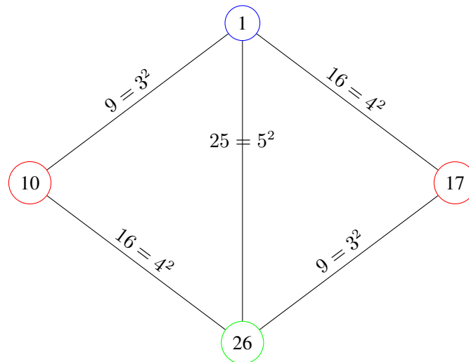
Figure 1. In any proper (x^2, 3) -coloring, \text{COL}(10) = \text{COL}(17)
