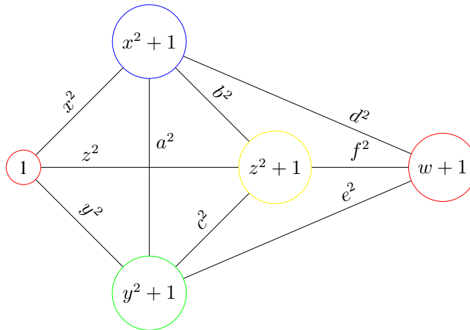
Figure 5. In any (x^2; 4) -proper coloring, \text{COL}(1) = \text{COL}(1 + w)
