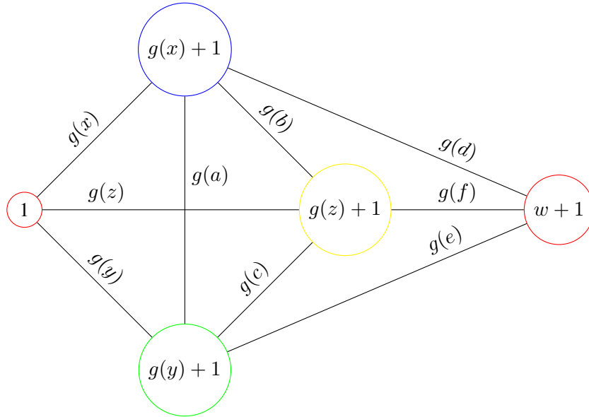
Figure 7. In any (g(x); 4) -proper coloring, \text{COL}(1) = \text{COL}(1 + w)
