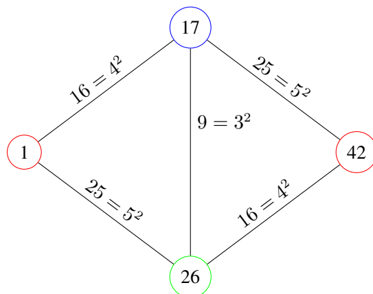
Figure 3. In any (x^2, 3) -proper coloring, \text{COL}(x) = \text{COL}(x + 41)
