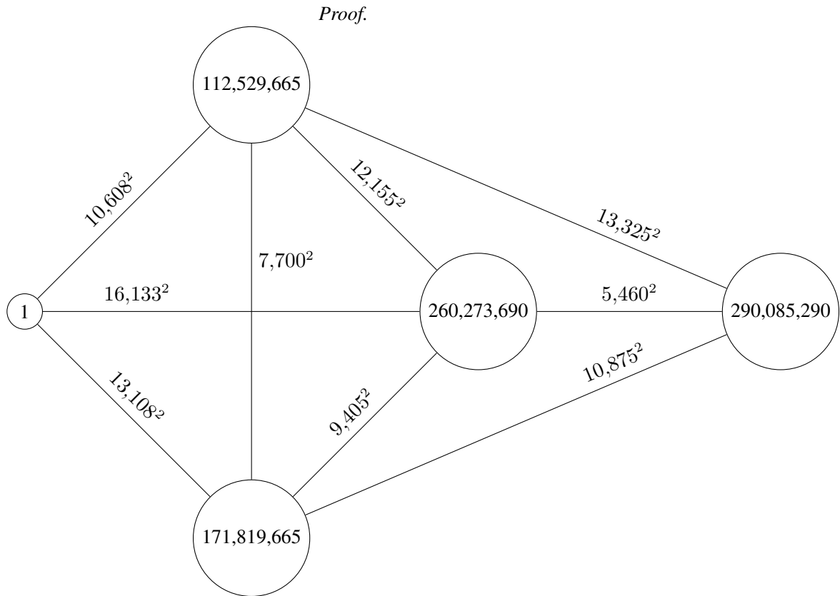
Figure 6. In any (x^2; 4) -proper coloring, \text{COL}(1) = \text{COL}(1 + 290,085,290)
