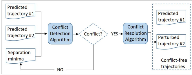
Figure 3: Overview of the CDR System.
