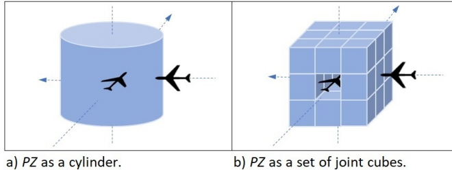
Figure 1: A sample crossing conflict and a PZ. (left) regular representation, (right) our unique representation.
