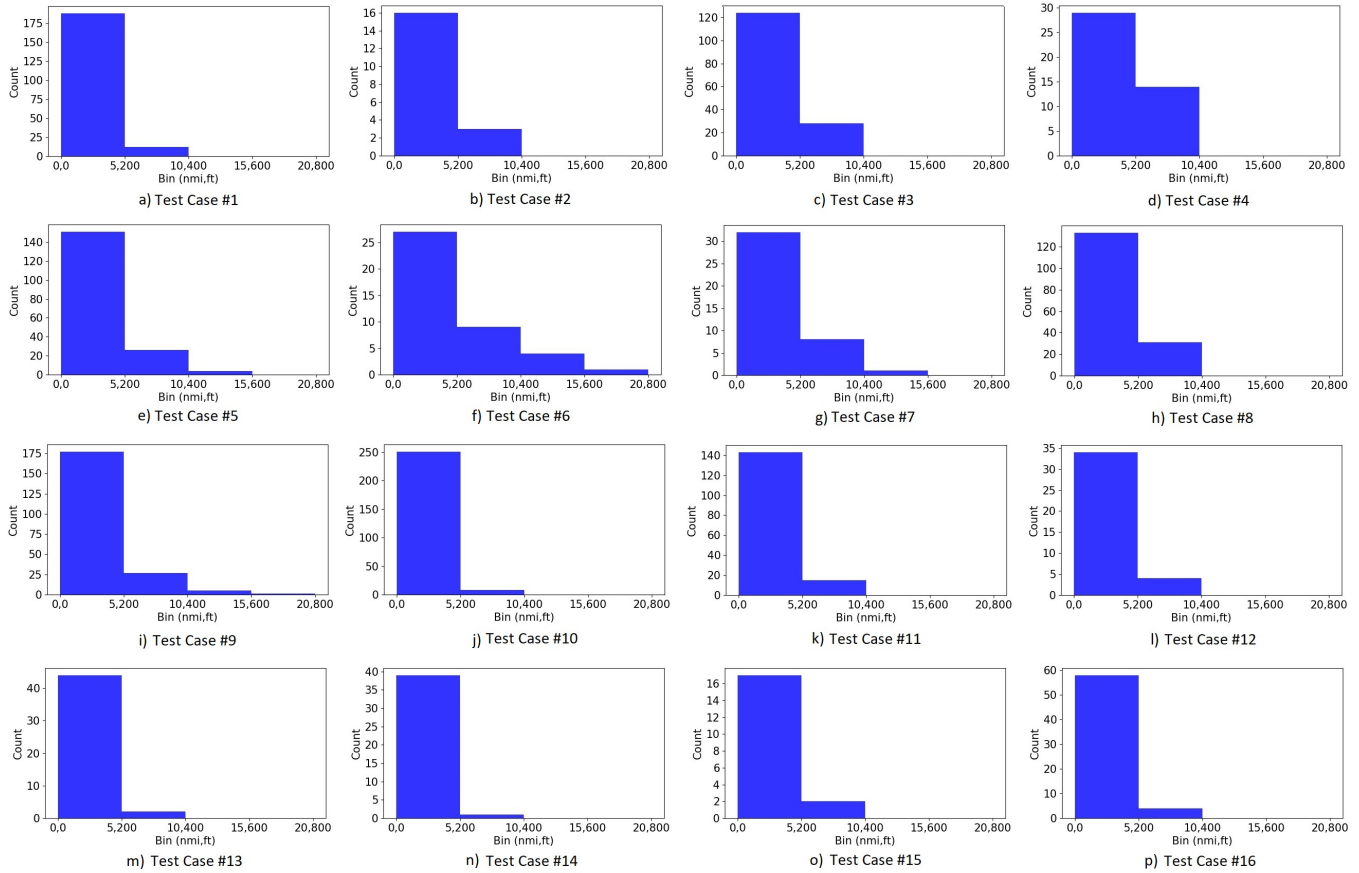
Figure 5: Conflict detection histograms showing how many conflicts were captured by our CDR System in each bin.
