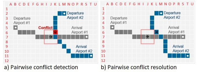
Figure 2: Simplified depiction of a pairwise CDR.
