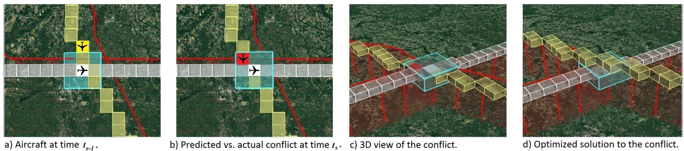
Figure 6: Illustration of a detected and resolved pairwise conflict by our system.
