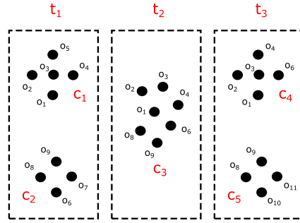
Fig. 3. Clusters observed during timespan [t_1 : t_3] .
