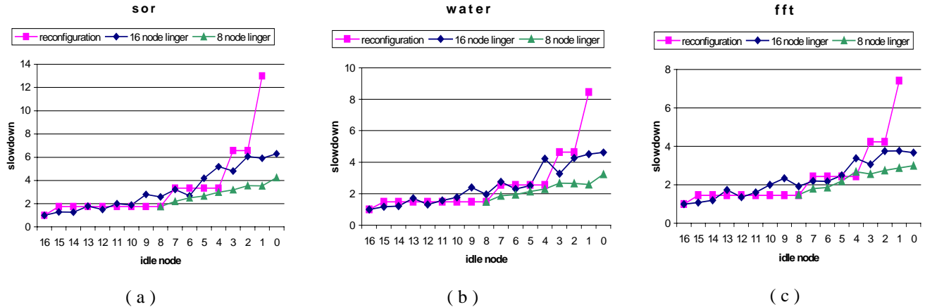
Figure 13: Linger-Longer vs. Reconfiguration for Shared-Memory Parallel Applications
