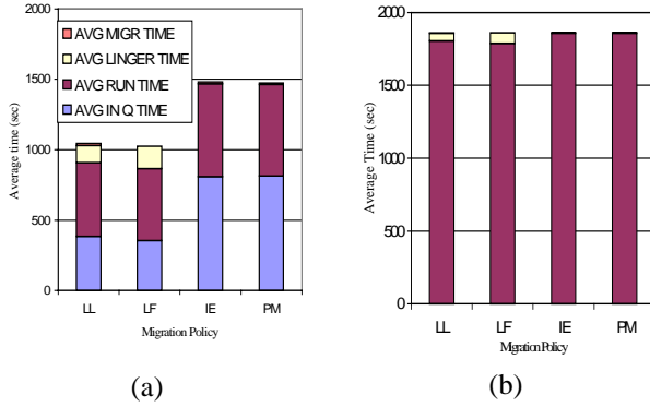
Figure 8: Average Completion Time
