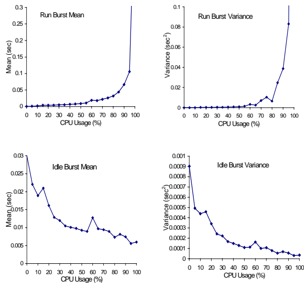
Figure 3: Workload Parameters
