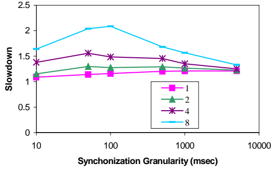
Figure 10: Synchronization Granularity vs. Slowdown
