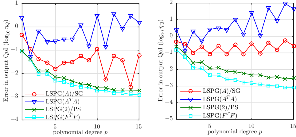
(a) Relative \ell^2 -norm of output QoI error \eta_Q with F = F_1 , n_o = 100 , and g(\xi) = g_1(\xi) = \sin(\xi) (b) Relative \ell^2 -norm of output QoI error \eta_Q with F = F_1 , n_o = 100 , and g(\xi) = g_2(\xi) = \xi
