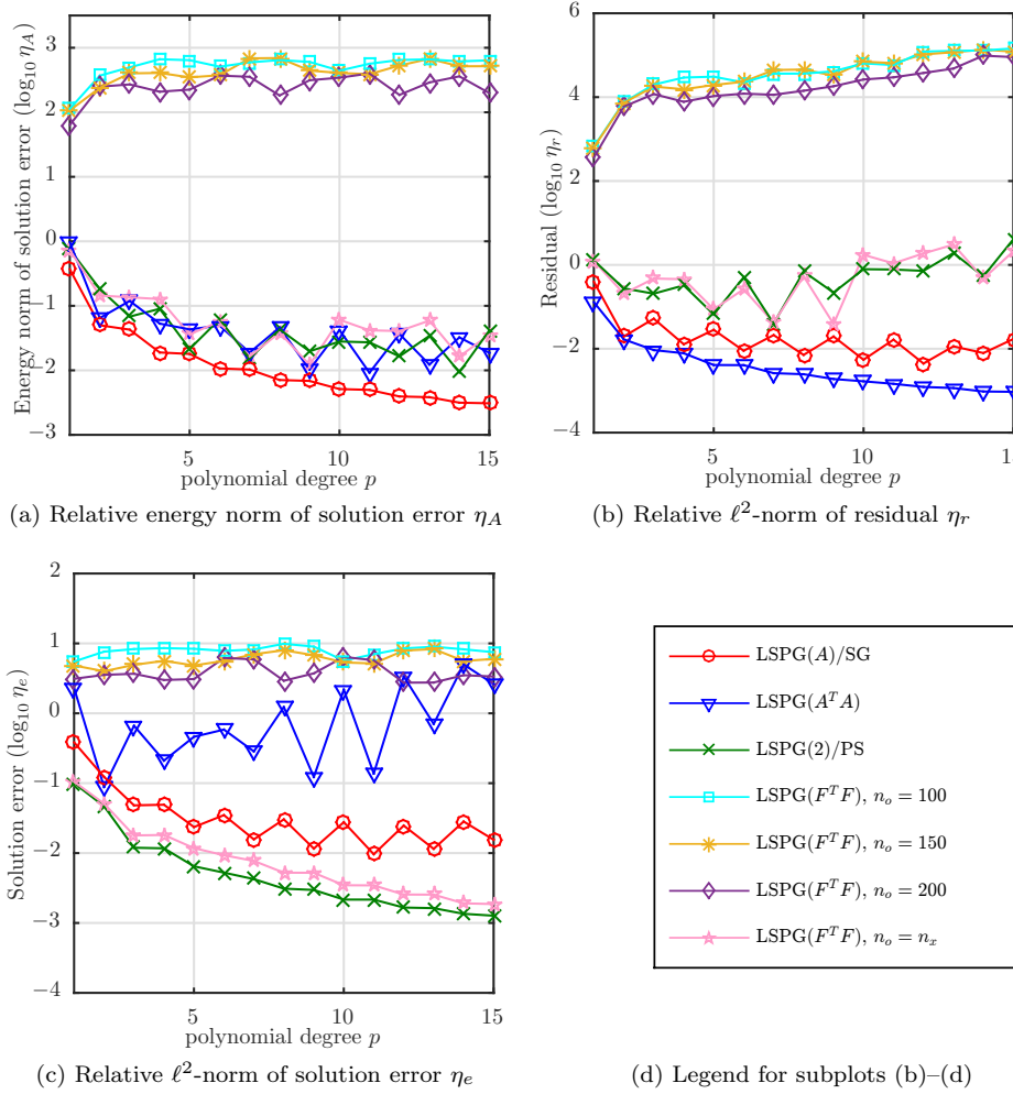
FIG. 5. Relative error measures versus polynomial degree for a varying dimension n_o of the output matrix F = F_1 for diffusion problem 2: lognormal random coefficient and random forcing. Note that LSPG( F^T F ) has controlled errors only when n_o = n_x , in which case \sigma_{\min}(F) > 0 .
