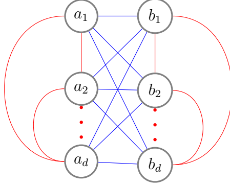
Figure 2: Edge Coloring of K_n , n Even, with Minimum Number of Monochromatic Triangles
