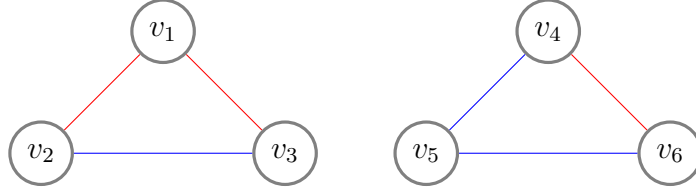
Figure 1: Mixed Triangles
