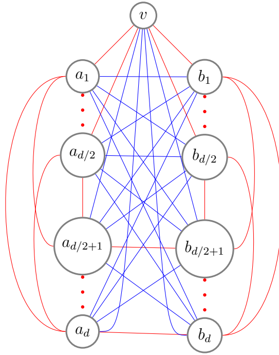
Figure 3: Edge Coloring of K_n , n Even, with Minimum Number of Monochromatic Triangles
