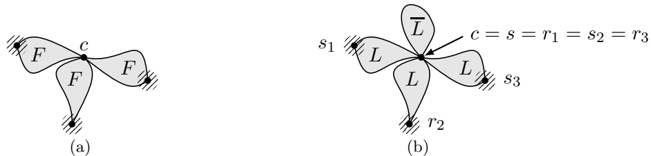
Figure 3: Connected component C' that might remain after removing a vertex cover S of G from G' , centered around a vertex c that has degree 3 in G and does not belong to S . (a) Naïve construction. (b) Final construction.
