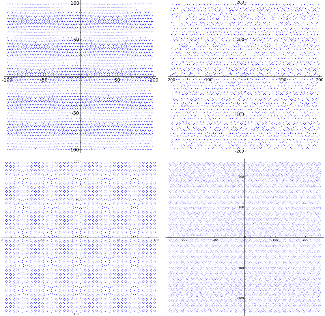
Figure 2: Top left: Q_{1+\varphi}(P_5) , the (1 + \varphi) -closure of a regular pentagon. Top right: Q_{\lambda_7}(P_7) , the \lambda_7 -closure of a regular heptagon. \lambda_7 \approx 5.049 and has minimal polynomial x^3 - 6x^2 + 5x - 1 . Bottom left: Q_{\lambda_6}(P_{12}) , the \lambda_6 -closure of a regular 12-gon. Bottom right: Q_{\lambda_7}(P_{14}) , the \lambda_7 -closure of a regular 14-gon
