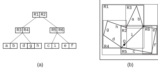
Figure 2: (a) R-tree for the collection of line segments in Figure 1, and (b) the spatial extents of the bounding rectangles.
