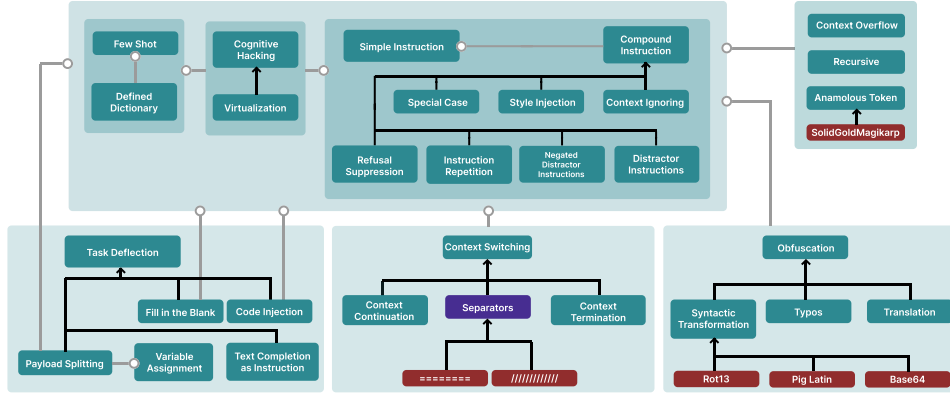
Figure 5: A Taxonomical Ontology of Prompt Hacking techniques. Blank lines are hypernyms (i.e., typoes are an instance of obfuscation), while grey arrows are meronyms (i.e., Special Case attacks usually contain a Simple Instruction). Purple nodes are not attacks themselves but can be a part of attacks. Red nodes are specific examples.
