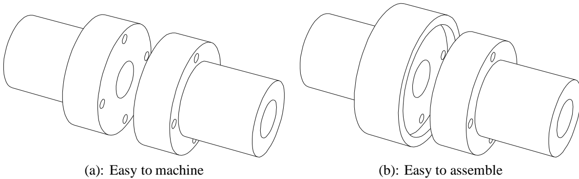
Figure 9: An example of conflicting requirements.
