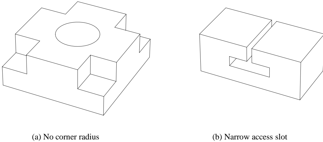
Figure 8: Design posing problem for machining.
