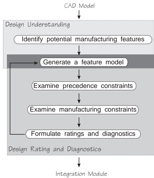
Figure 7: Critiquing Procedure
