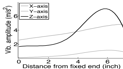
Figure 10: Vibration highest at a specific phone location.
