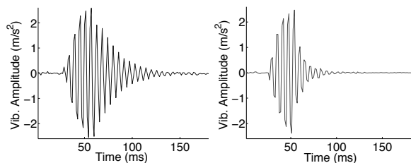
Figure 11: (a) Ringing effect in the channel. (b) Reduced ringing using a braking voltage.
