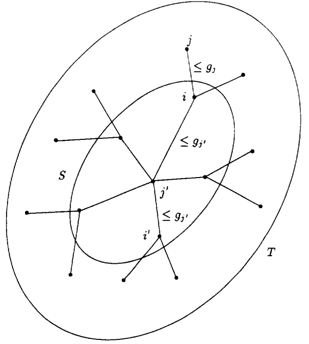
Figure 1: Rounding the solution near j' , where edges correspond to positive components of \hat{x}
