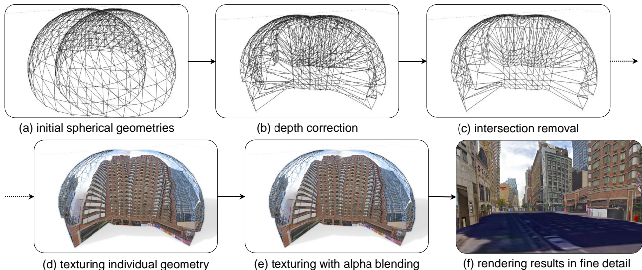
Figure 2: Our rendering pipeline for fusing 360° images in fine detail. (a) We start by generating spherical geometries to represent the 360° images. (b) In the vertex shader, we correct the depth value for each vertex by sampling the depth maps with its spherical coordinates. (c) In the fragment shader, we discard the pixels in the intersection of the adjacent geometries. (d) Texturing individual spheres with the corresponding 360 images may leave a visible seam. (e) Texturing the spheres with a weighted average according to the position to the camera yields a smoother result. (f) Finally, we interactively texture the ground plane with the corresponding satellite images, apply Gaussian filters in occluded regions, and allow the users to freely walk along the street while streaming the next street views on the go.
