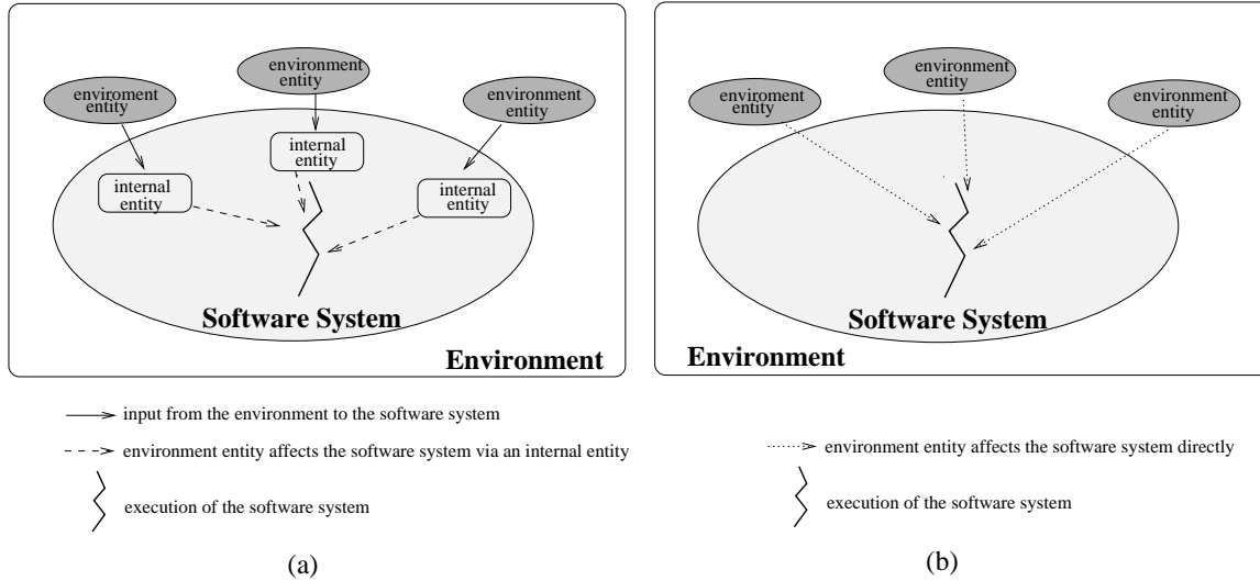
Figure 1. Interaction Model
